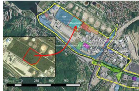
Trieste Ezit11 field aerial view
